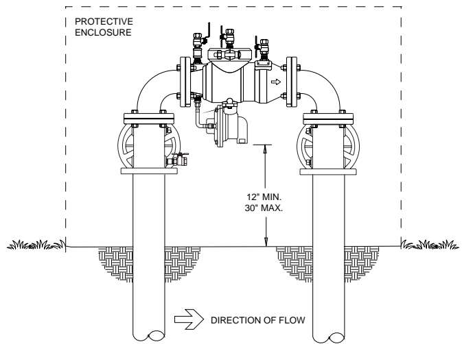
OUTDOOR INSTALLATION
