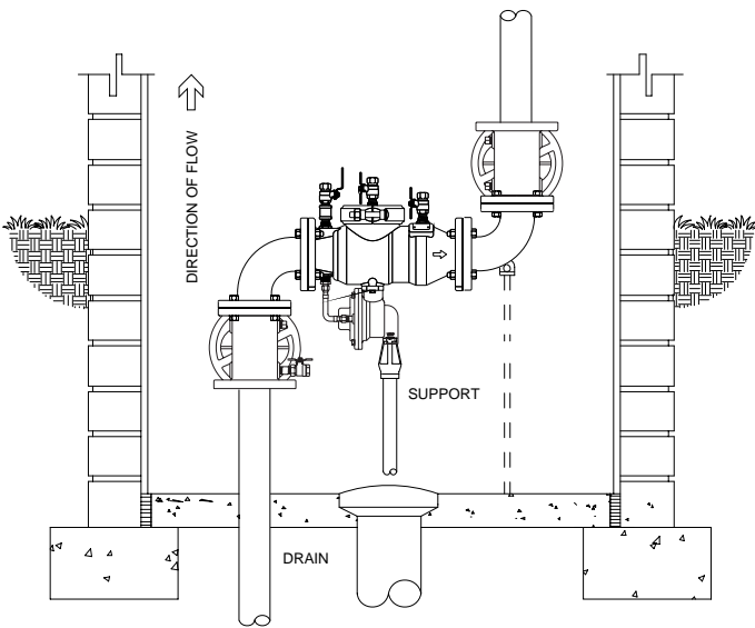
INDOOR INSTALLATION
